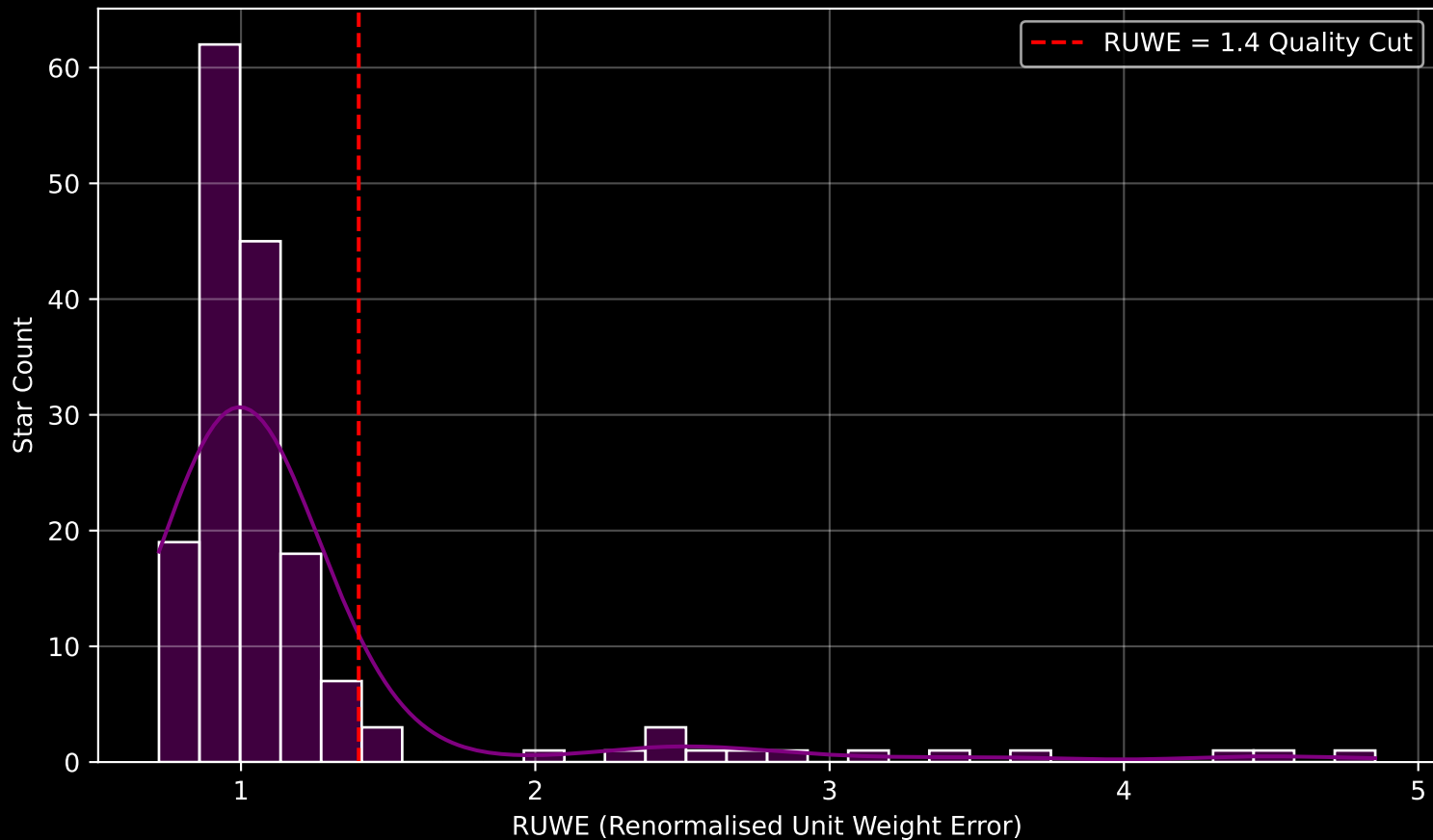
GAPOGEE DR17 Field [CVZ_OB10_btx] RUWE Distribution (n= 168)
