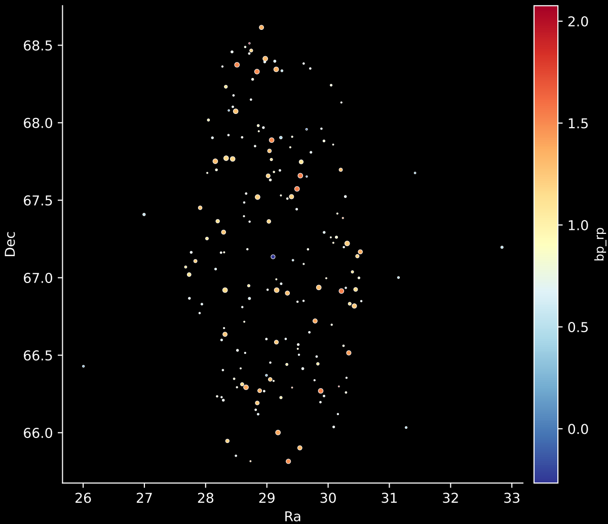
APOGEE DR17 Field: [CVZ_OB10_btx] Stars: 181
