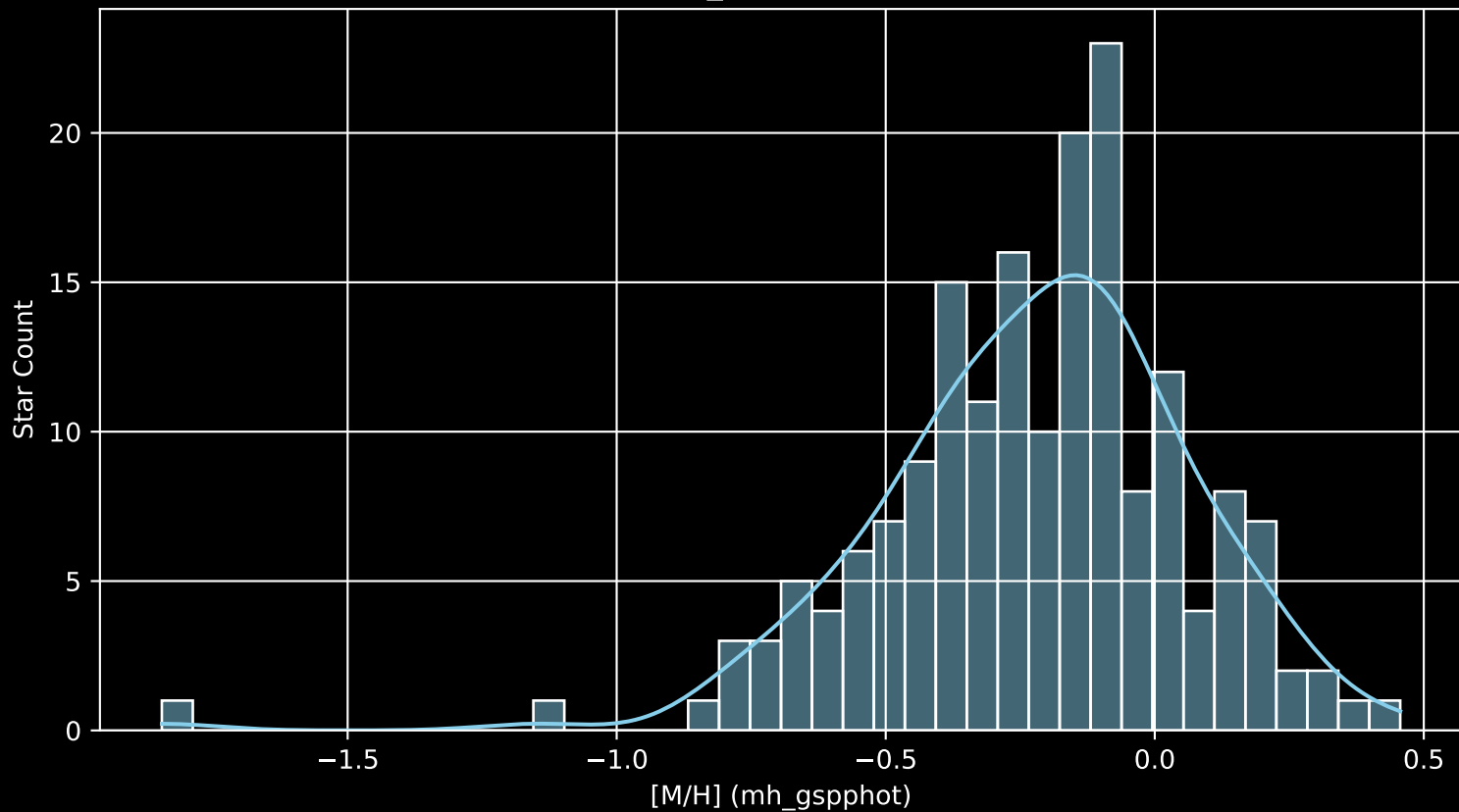
APOGEE DR17 Field: [CVZ_OB10_btx [M/H] (mh_gspphot) (n= 180)
