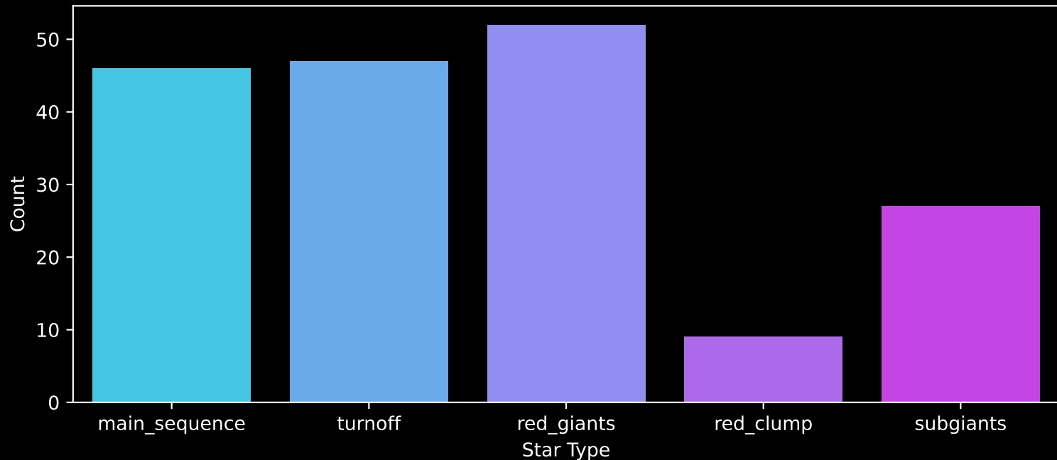
APOGEE DR17 Field: [CVZ_OB10_btx] Count plot of Star Type
