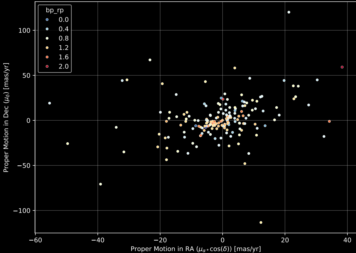
APOGEE DR17 Field: [CVZ_OB10_btx] Proper Motion Diagram (n= 181)
