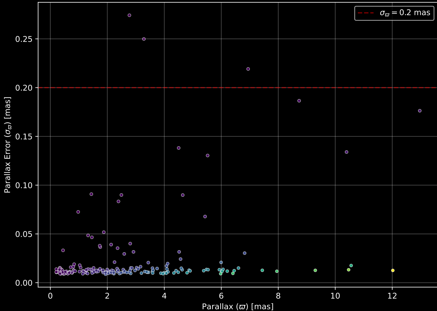
APOGEE DR17 Field: [CVZ_OB10_btx] Parallax Quality (n= 181)
